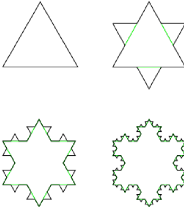
Koch Snowflake which includes many Koch curves forming all the edges
